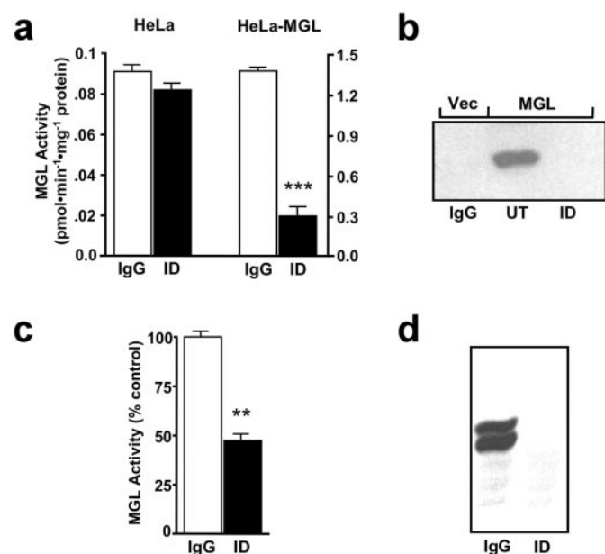
Fig. 3. Effects of MGL immunodepletion in rat brain soluble fraction. a , MGL enzyme activity in vector- (left) and MGL-infected (right) HeLa cells before and after MGL immunodepletion. b , Western blot analysis of MGL-overexpressing HeLa supernatant before (UT) and after immunodepletion (ID). No MGL-like immunoreactivity was detected in supernatant from vector-infected (Vec) or MGL-immunodepleted HeLa cells. c , MGL enzyme activity in rat brain soluble fraction before (□) and after (■) MGL immunodepletion. d , MGL-like immunoreactivity is absent in MGL-immunodepleted (ID) but not rabbit IgG-treated soluble fractions. **, P < 0.01 ; ***, P < 0.001 ; Student's t test ( n = 6 ).
