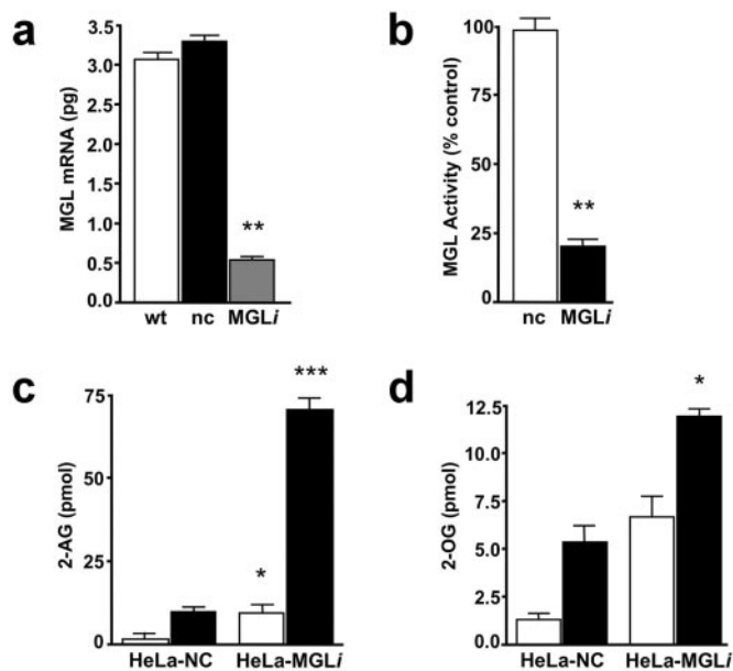
Fig. 1. RNAi-mediated suppression of MGL expression increases 2-AG content in HeLa cells. a , real-time quantitative PCR of MGL mRNA expression in wild-type HeLa cells (□), HeLa-NC cells (negative control) (■), and HeLa-MGLi cells (▨) ( n = 5 ). Initial quantities were determined using glyceraldehyde-3-phosphate dehydrogenase as a standard. b , MGL activity in HeLa-NC (□) and HeLa-MGLi (■) ( n = 3 ). 2-AG ( c ) and 2-OG ( d ) content in HeLa-NC and HeLa-MGLi cells incubated with vehicle (□) or ionomycin ( 2 \mu\text{M} for 15 min) (■). Results are representative of two independent experiments performed in triplicate. *, P < 0.05 ; **, P < 0.01 ; ***, P < 0.001 ; one-way analysis of variance ( a , c , and d ) and Student's t test ( b ) ( n = 6 ).
