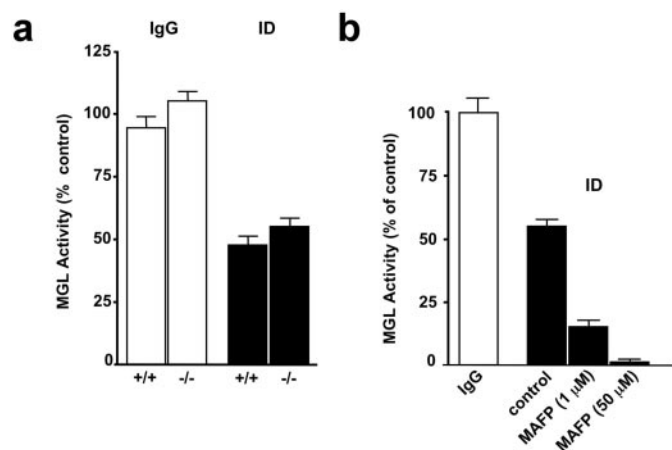
Fig. 4. FAAH does not contribute to the 2-AG-hydrolyzing activity in rat brain supernatant. a , 2-AG-hydrolyzing activity in rabbit IgG-treated (□) and MGL antibody-treated (■) brain supernatants of wild-type and faah -/- mice ( n = 3 ). b , residual 2-AG-hydrolyzing activity in MGL-immunodepleted (ID) fractions is inhibited by MAFP ( n = 3 ).
